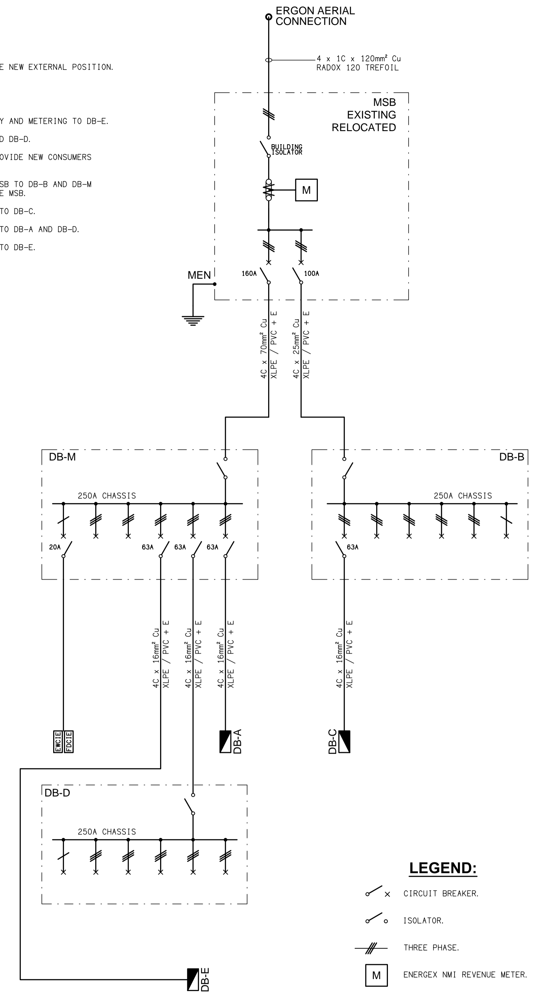
SCHEMATIC POWER CONFIGURATION NOT TO SCALE
